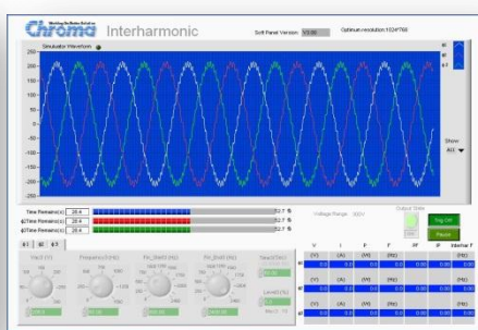
Interharmonic Test
